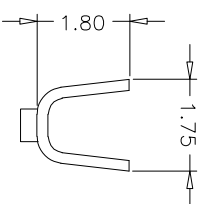
Sections C-C
